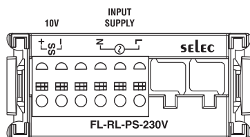
Figure 4.1 : FL-RL-PS-230V wiring
